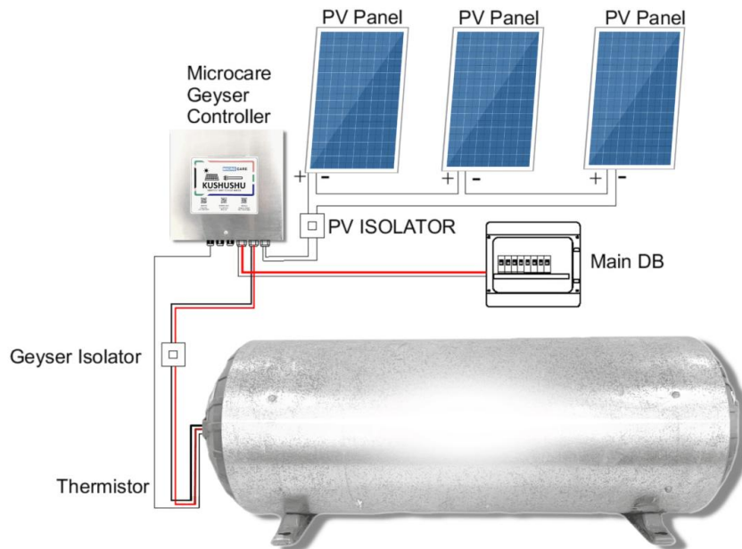
Figure 3. Schematic of a PV2Heat system from Microcare [7].
